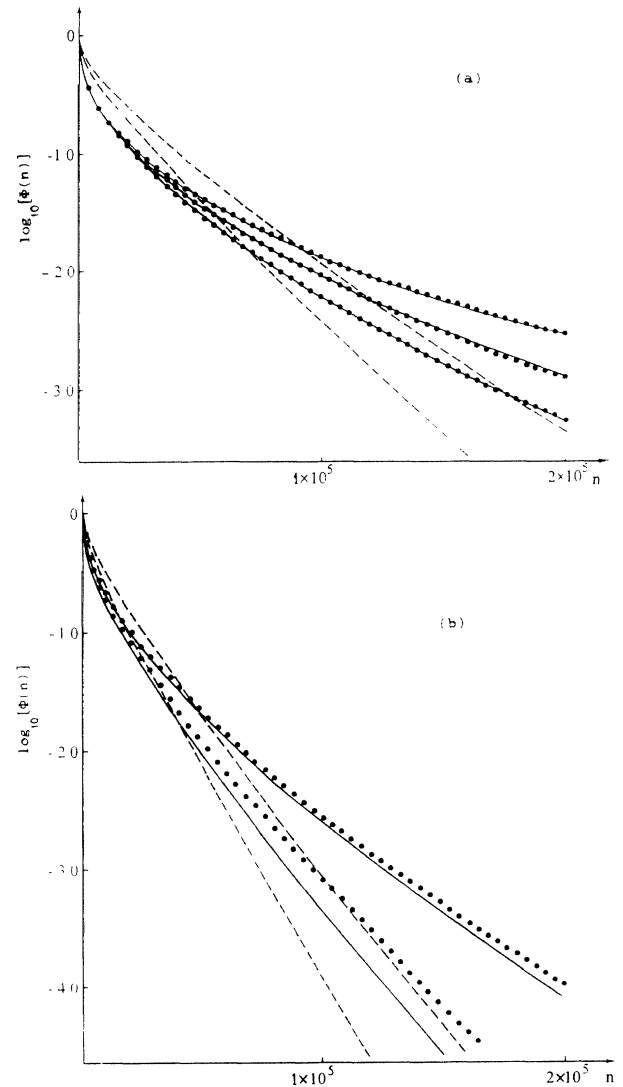
FIG. 1. Decay of \Phi(n) for the trap concentration C=0.01 at various values of the quasi-one-dimensionality degree \delta_2 . The circles denote the MC simulation, the solid lines the results from Eq. (5), and the dashed lines the results from Eq. (8). (a) From top to bottom: \delta_2 \leq 10^{-7} ; \delta_2 = 5 \times 10^{-6}, 10^{-5} . The thin line is the exact decay form of \Phi(n) for strictly 1D migration as obtained in [8]. (b) From top to bottom: \delta_2 = 2 \times 10^{-5}, 4 \times 10^{-5} .
