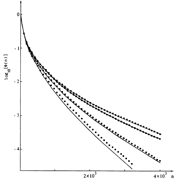
FIG. 2. Decay of \Phi(n) for the trap concentration C = 0.1 at various values of the quasi-one-dimensionality degree \delta_2 . The circles denote the MC simulation, and the solid lines the model results from Eq. (5). The thin line is the exact decay form of \Phi(n) for strictly 1D migration as obtained in [8]. From top to bottom: \delta_2 \leq 5 \times 10^{-6} ; \delta_2 = 10^{-4} , 5 \times 10^{-4} , 10^{-3} .
